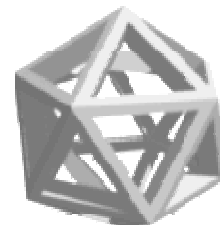
icosahedron
